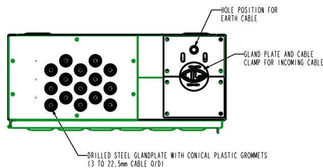
FRONT VIEW WITH DOOR AND INCOMING CABLE SCREEN REMOVED
