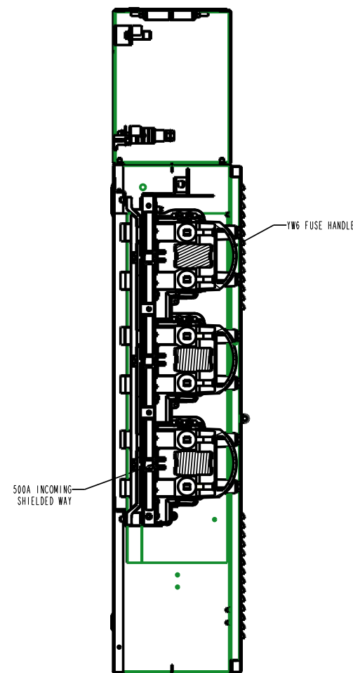
SECTION C-C SHOWING 500A INCOMING SHIELDED FUSEWAY
